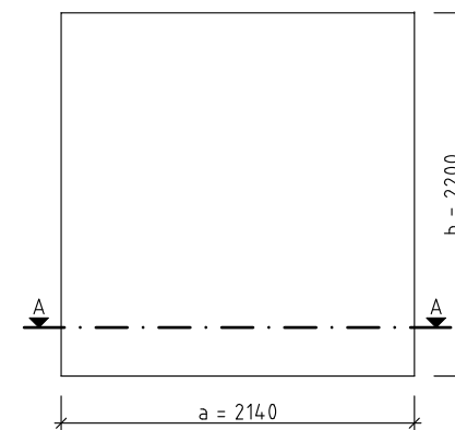
Fundamentplan M 1:50
